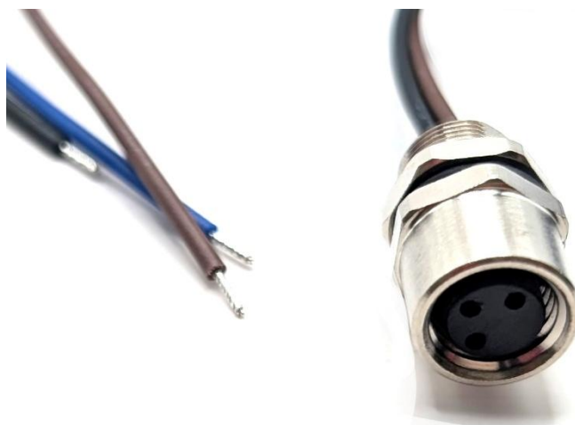
Pin Out
